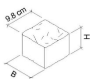
FRIEDA® Pflasterstein 9.8 × 9.8 × 7 cm
